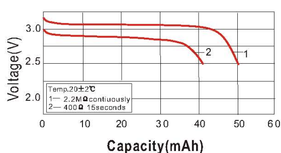
Pulse Discharge Characteristic
