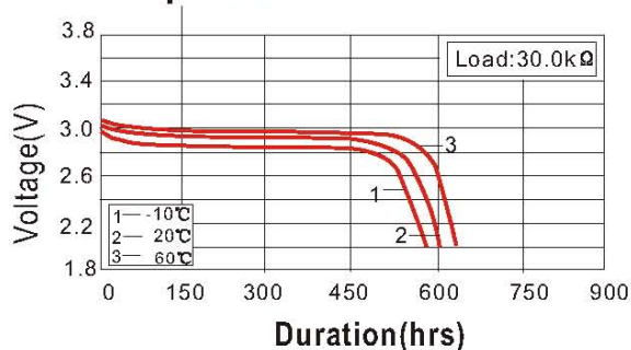
Temperature Characteristics
