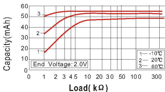
Load-capacity characteristic
