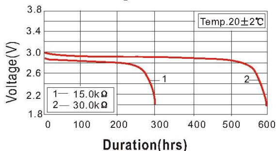
Discharge characteristics
